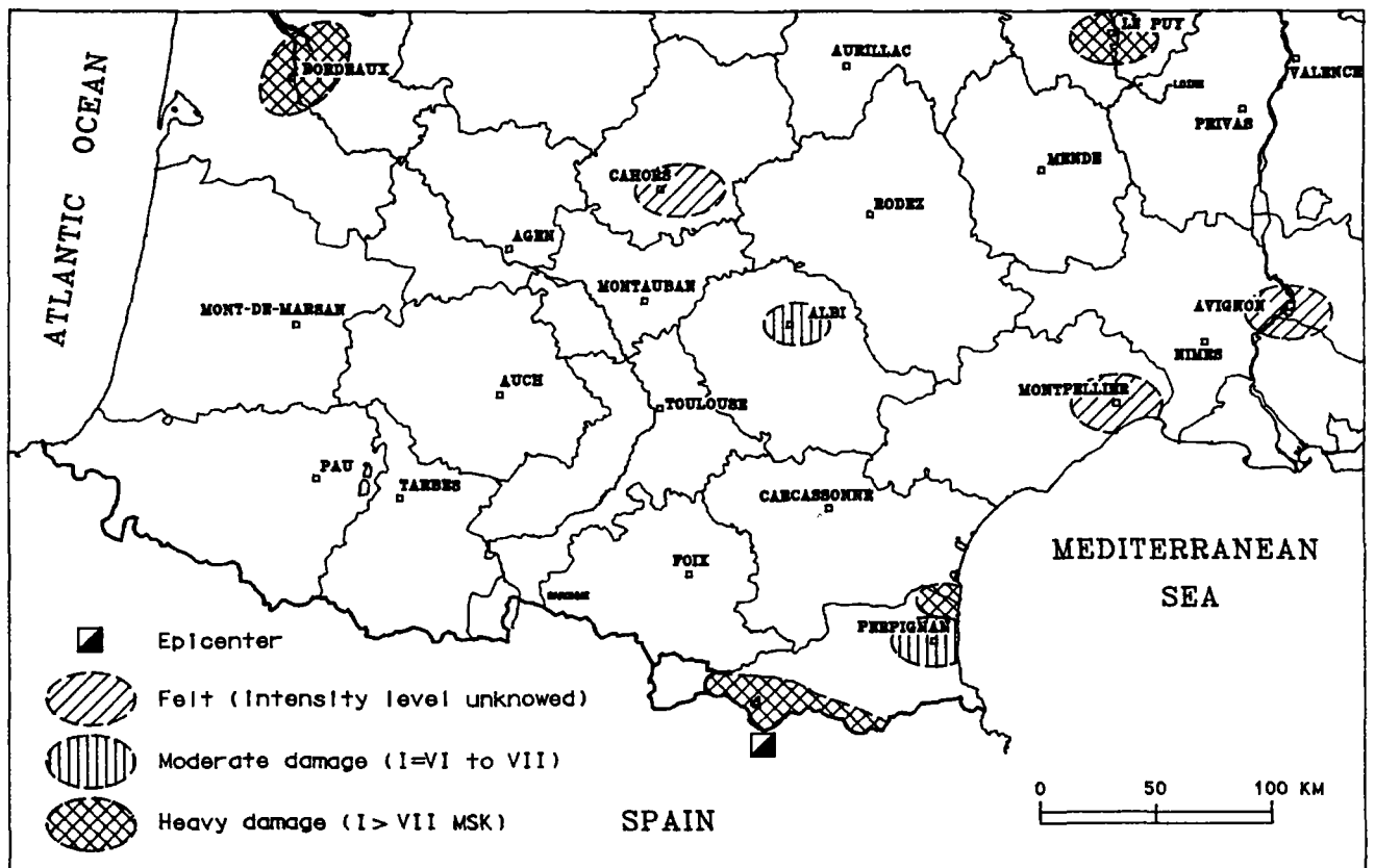
1428 February 2 nd event Southwest part of France : location plan (1989)
